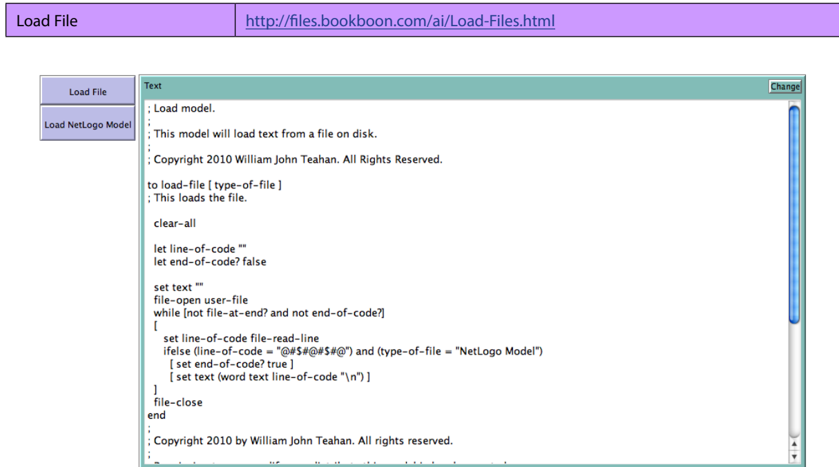
Figure S-3.5.3. Screenshot of the Interface for the Load File model after the Load NetLogo Model button has been pressed, and the Load-File.nlogo file has been loaded.
