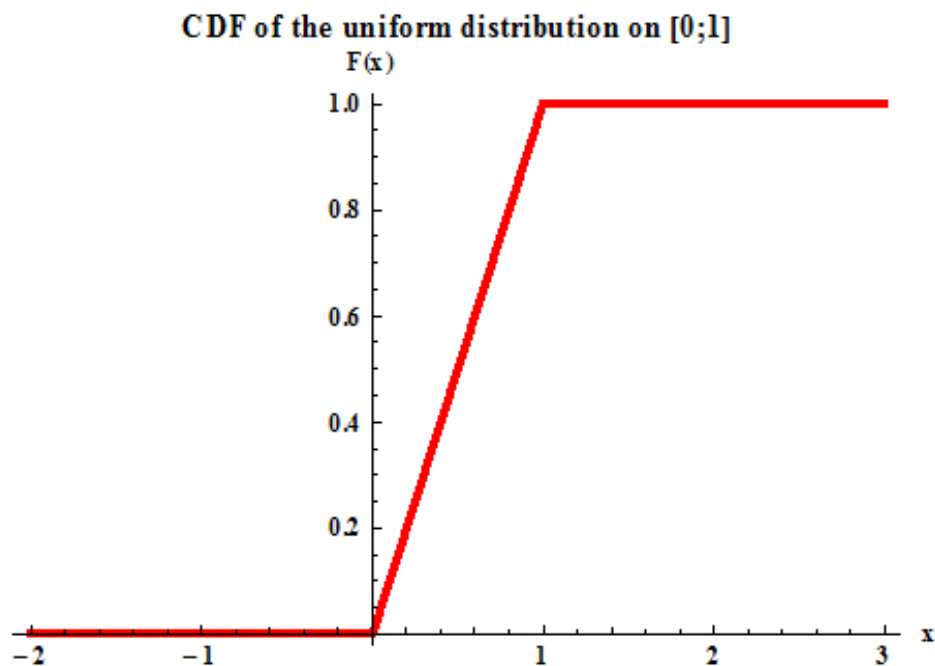
Figure 3.2: CDF of the uniform distribution on [0; 1]
